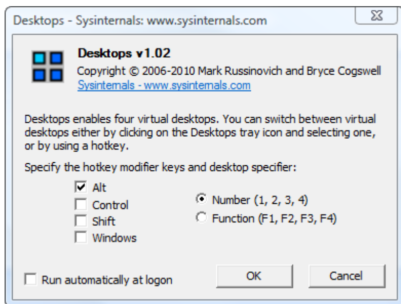
Configuration Dialog
